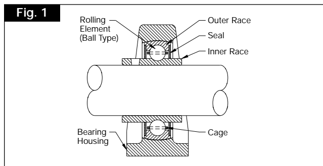
Fig. 1 Cutaway View of a Ball Bearing Unit
