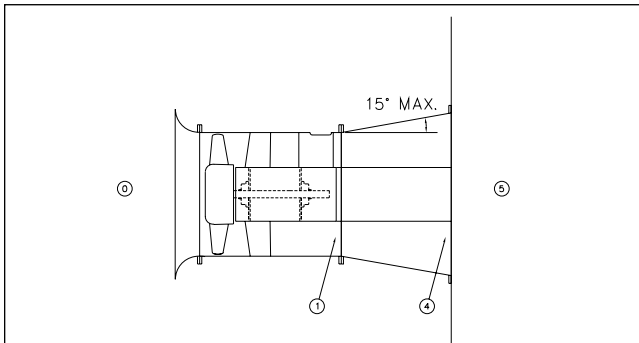
Figure 6. Axial Fan Connected to a Non-Ducted Outlet Cone with Center Body
